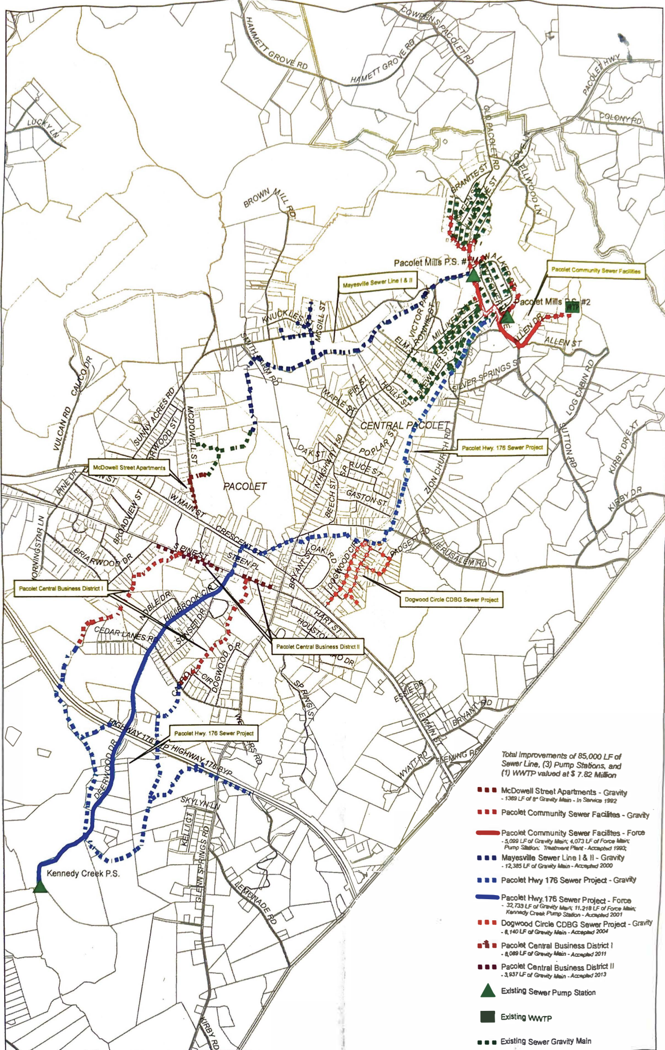
Pacolet Area Sewer 1991-2022 NOT TO SCALE
